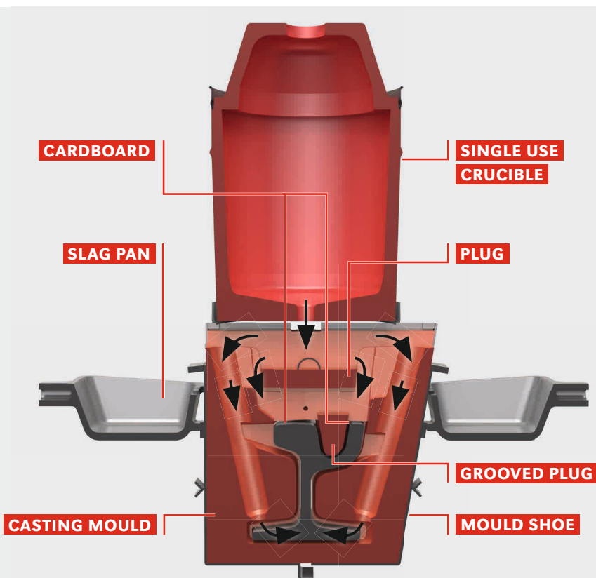
Central pouring/combined casting system
